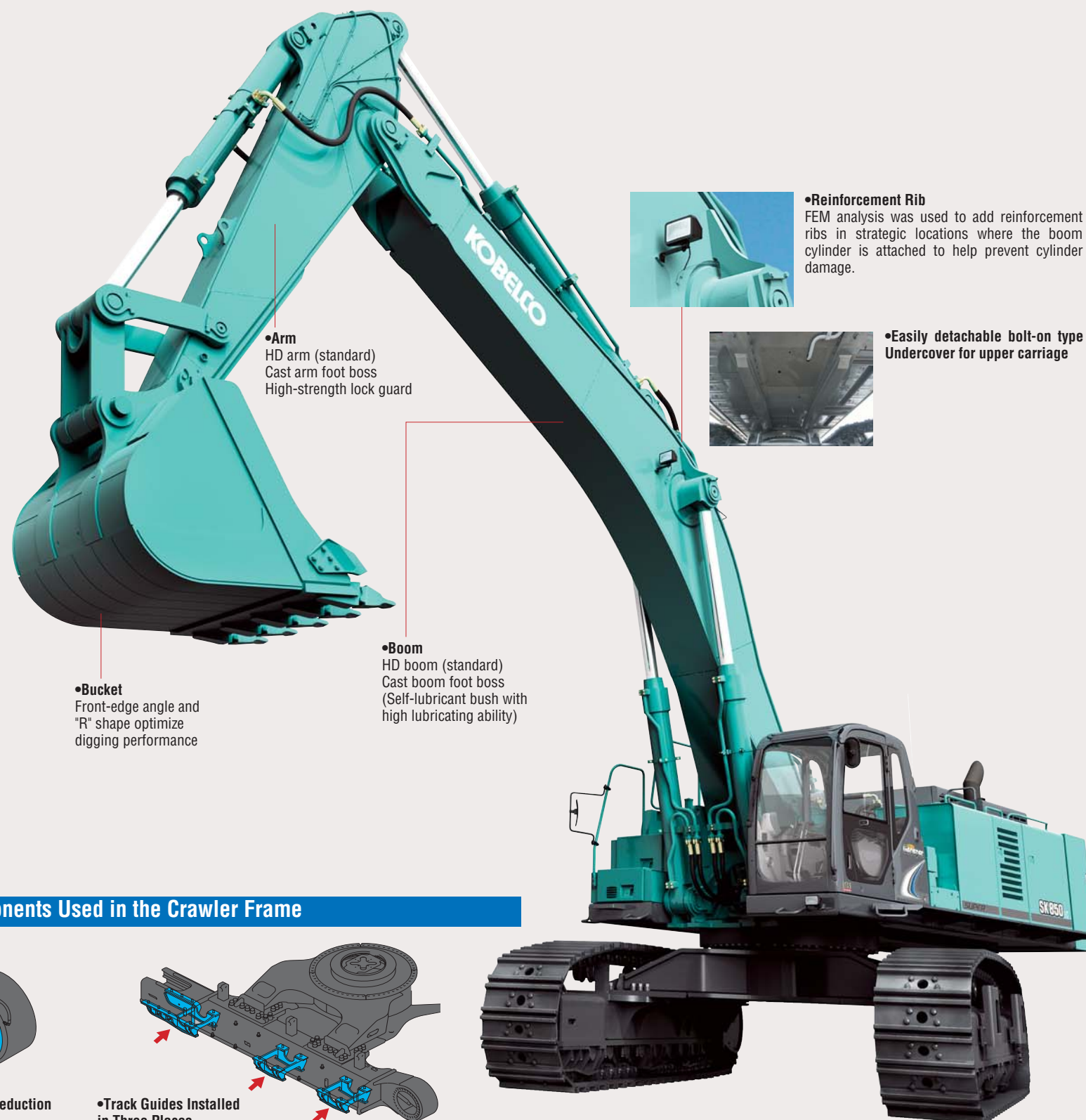
*FEM (Finite Element Method) Method of numerical analysis used in structural mechanics
