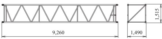
9.1 m Boom Insert Weight: 745 kg
