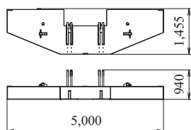
Counterweight (1) Weight: 9,800 kg
