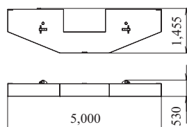
Counterweight (2) Weight: 9,610 kg
