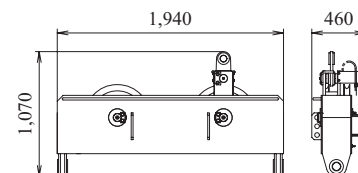
Lower Spreader (for Tower) Weight: 410 kg
