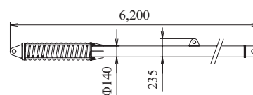
Backstop (for Tower) Weight: 420 kg / 1 piece
