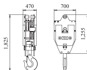
70 t Hook Weight: 1,200 kg
