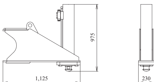
Translifter Weight: 1,220 kg / 4 pieces
